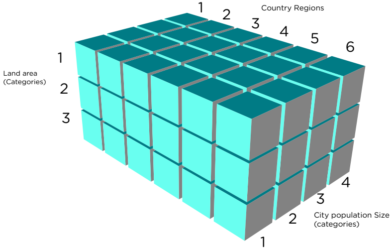
Figure 1: Visualization of the list of cities combined into 72 boxes, each box corresponding to one of six country regions, one of three city-area-size ranges, and one of four city-population-size ranges ( 6 \times 3 \times 4 = 72 )
